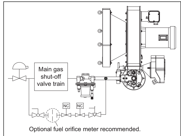
Figure 3.7. Pilot Start (Optional)
