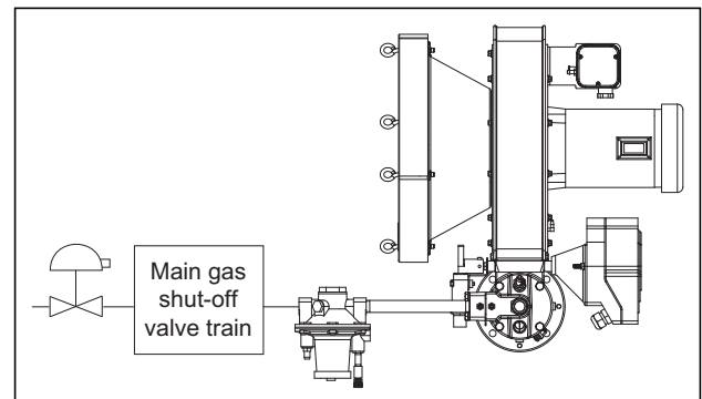
Figure 3.6. Low Fire Start
