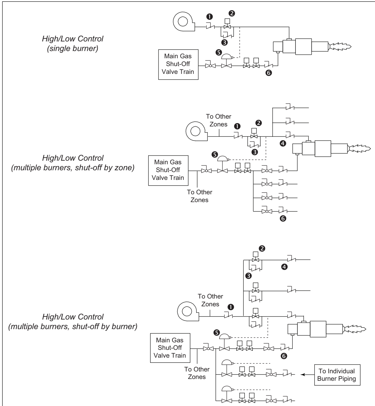
Figure 3.1 High/Low Control
