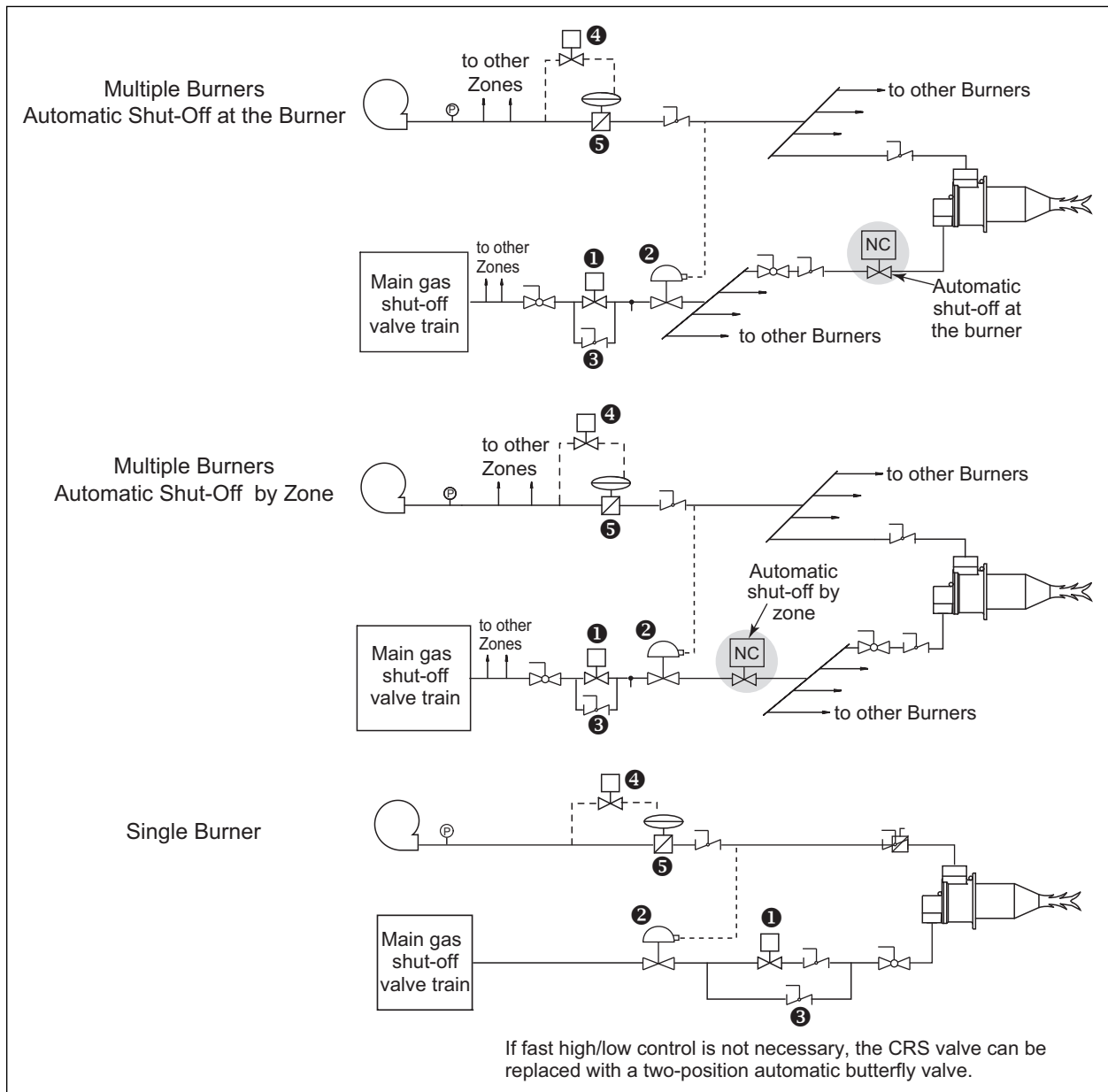
Figure 3.3 High/Low Air & Gas Control (Pulse Firing)
