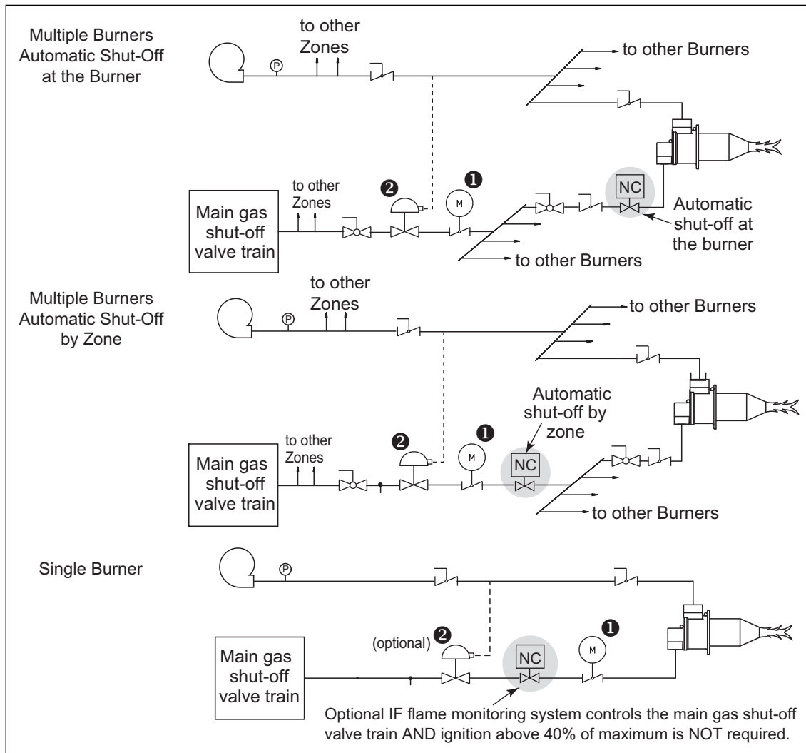
Figure 3.2 Modulating Gas with Fixed-Air Control
