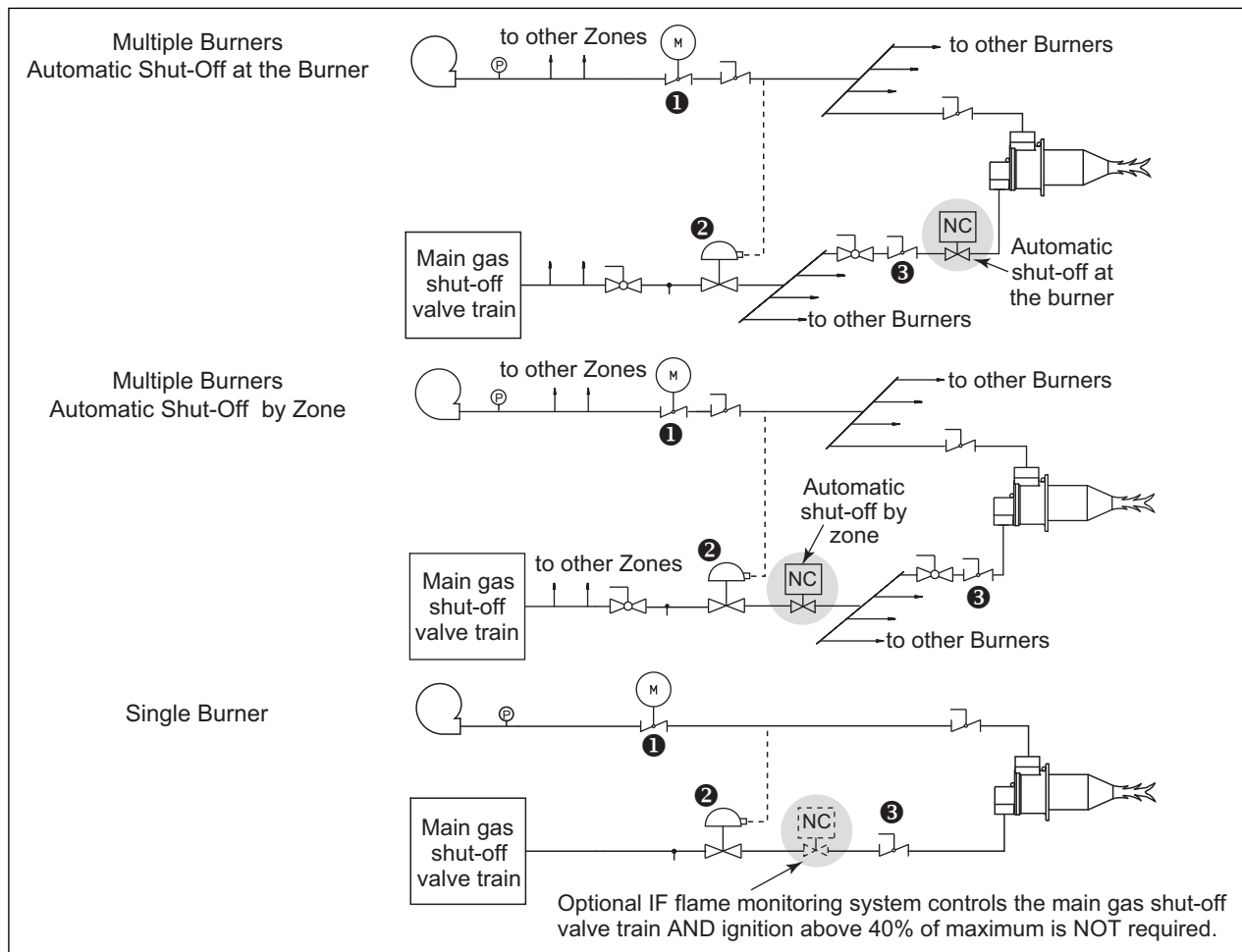
Figure 3.1 Modulating Gas & Air (On-Ratio Control or Excess Air @ Low Fire)
