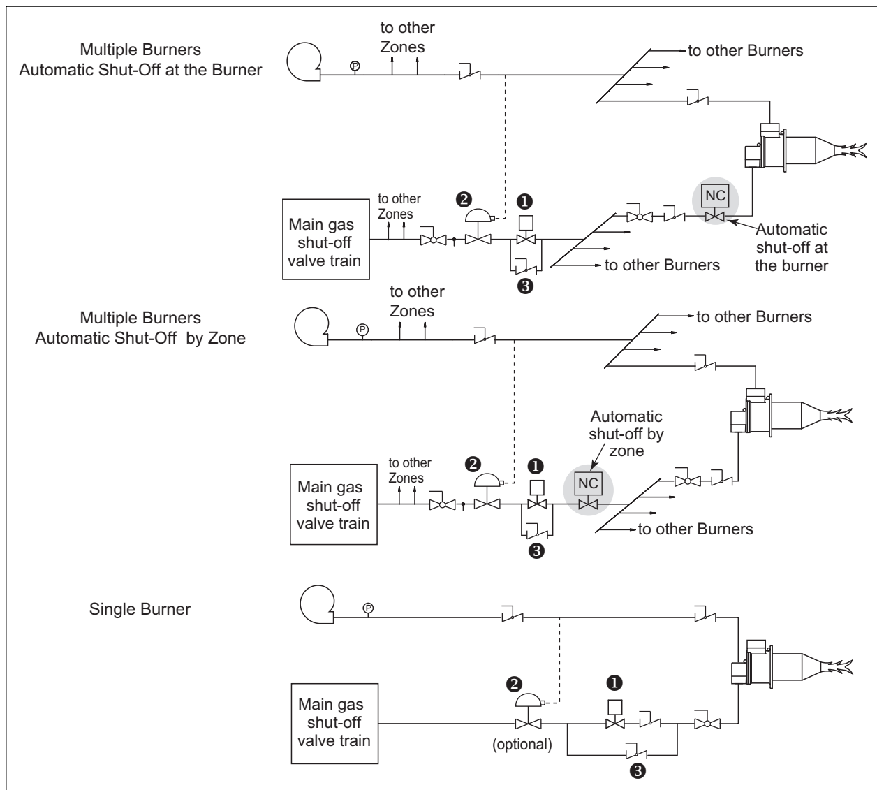
Figure 3.4 High/Low Gas with Fixed-Air Control
