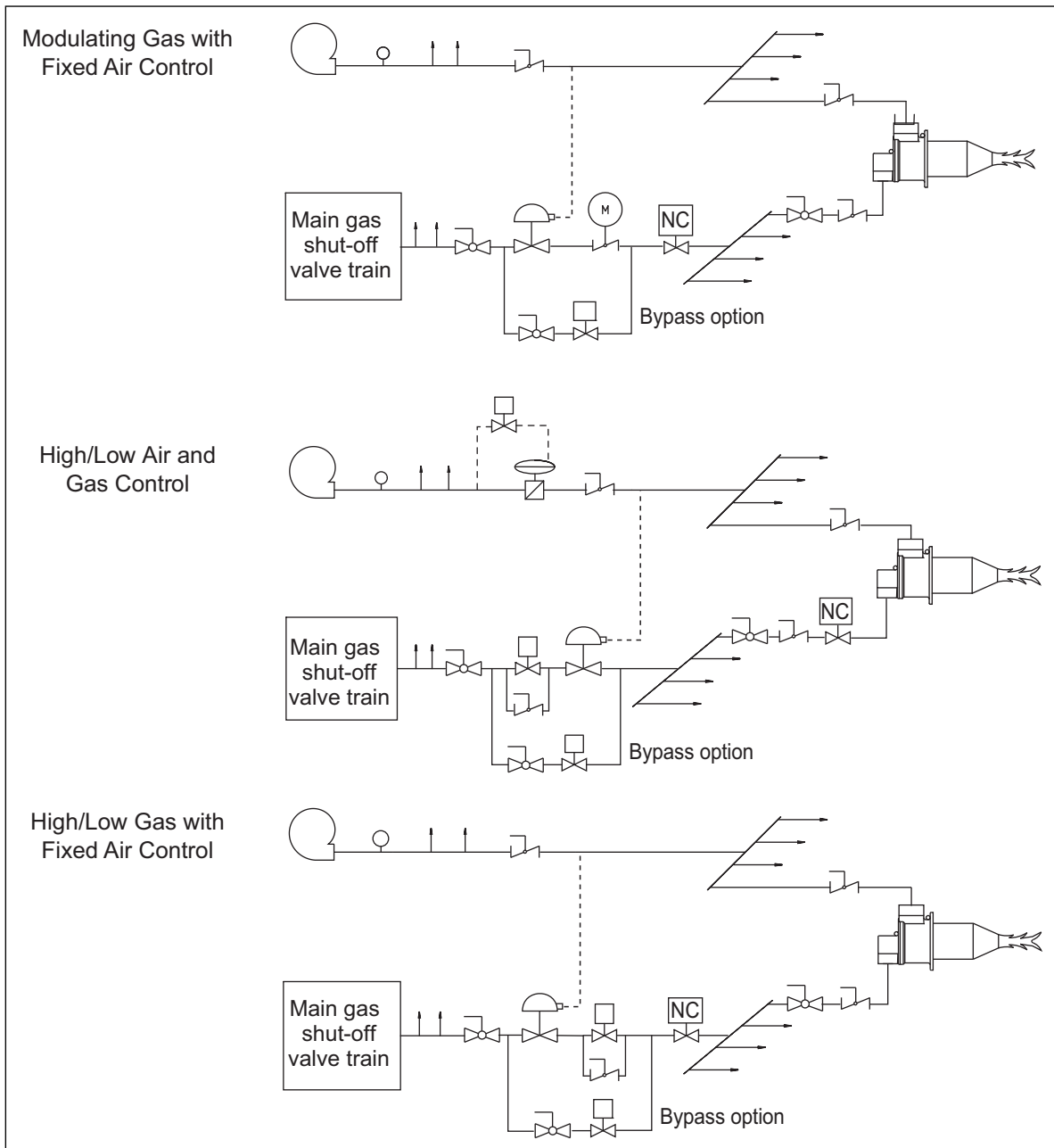
Figure 3.5 Bypass Start Gas Circuit Schematics
