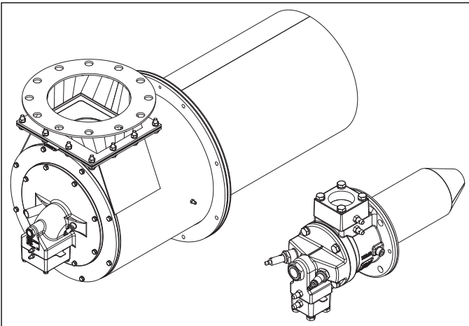
Figure 1.1. Eclipse ThermJet Burner
