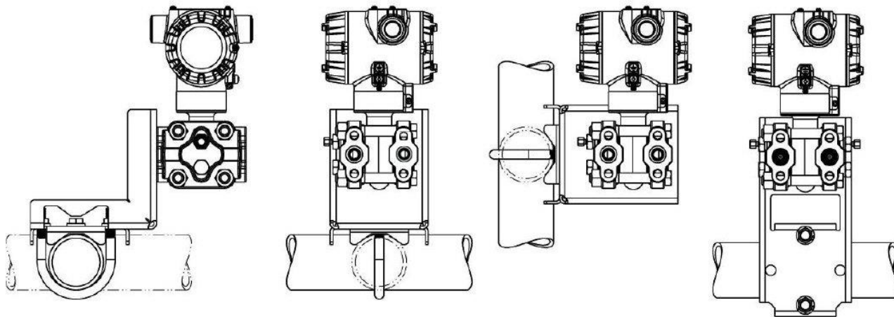
Figure 4 – Mounting Configurations
