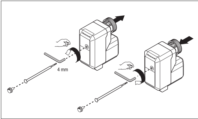
Fig. 6. Manual operation
